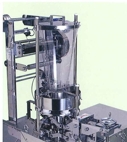
Variable volume type turn-table filling device
